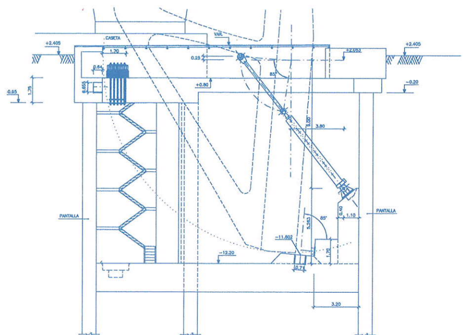
Fig. 8. Alzado del recinto-pila. Fig. 8. Cross section of the pits.
